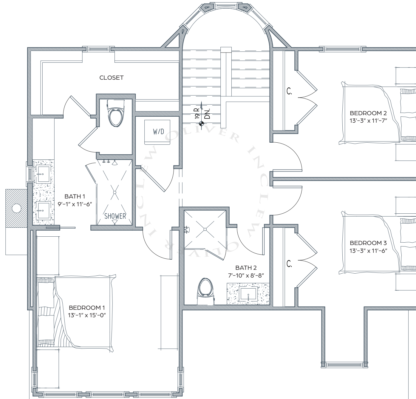
SECOND FLOOR
