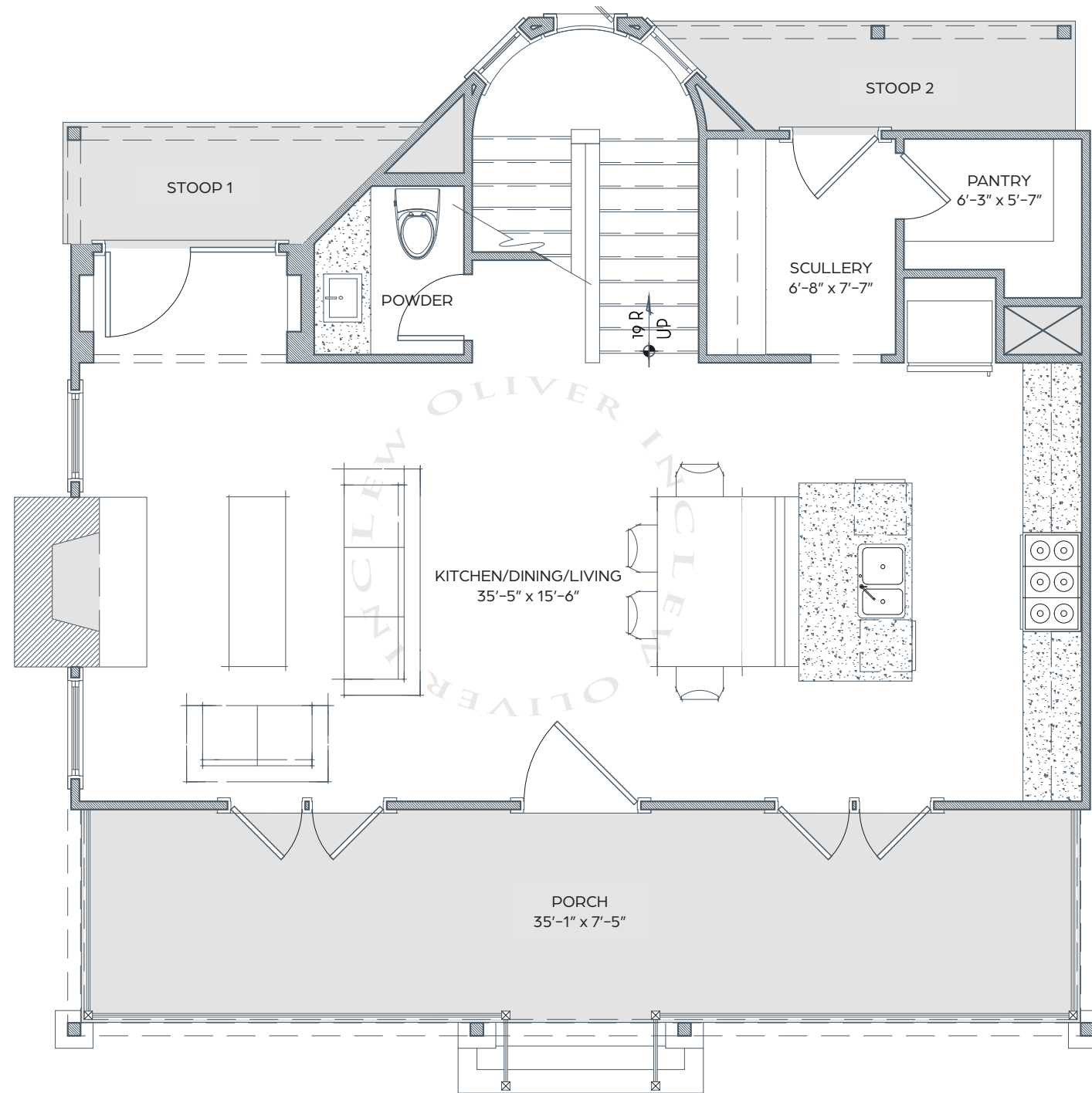
FIRST FLOOR
