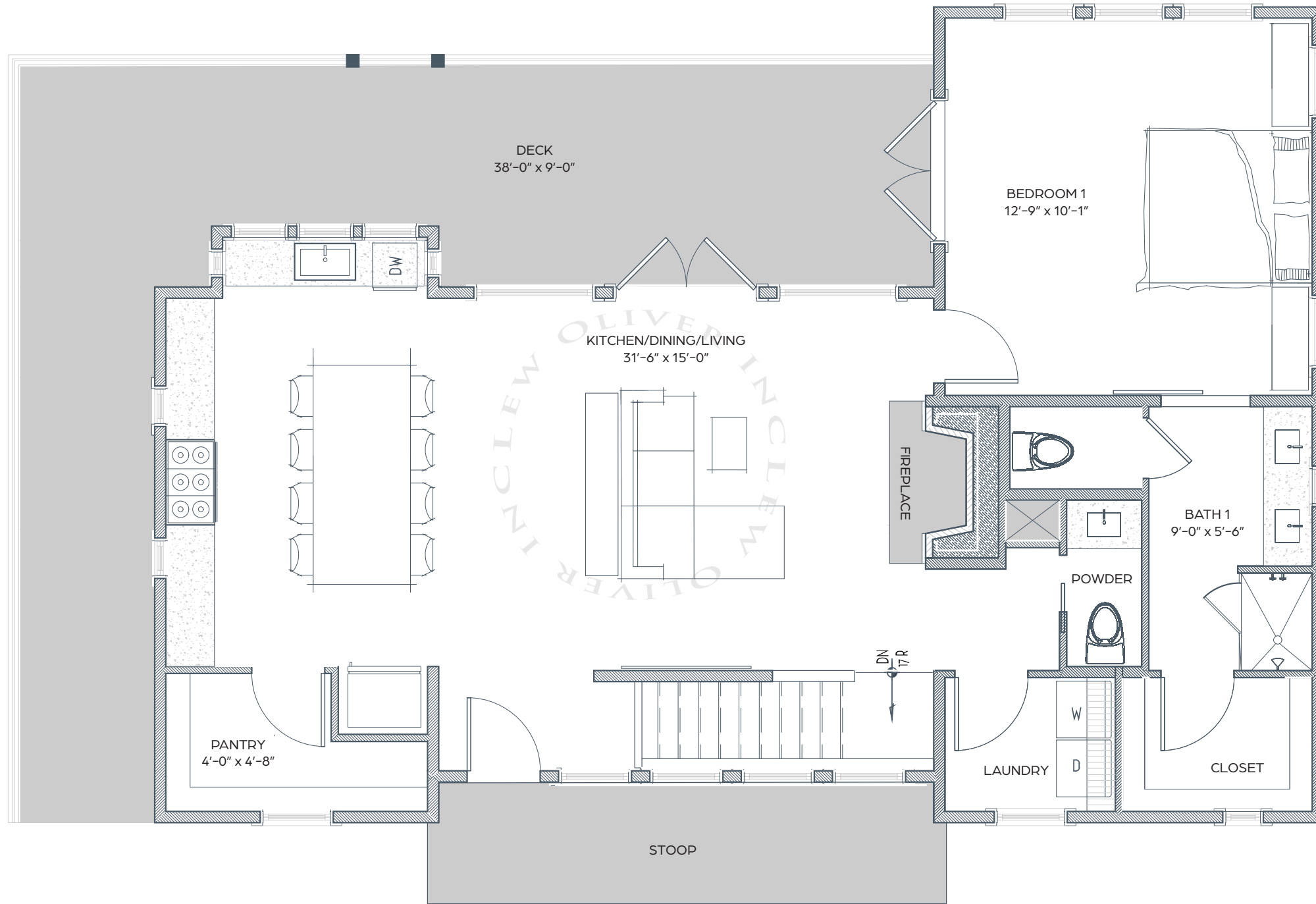
MAIN FLOOR
