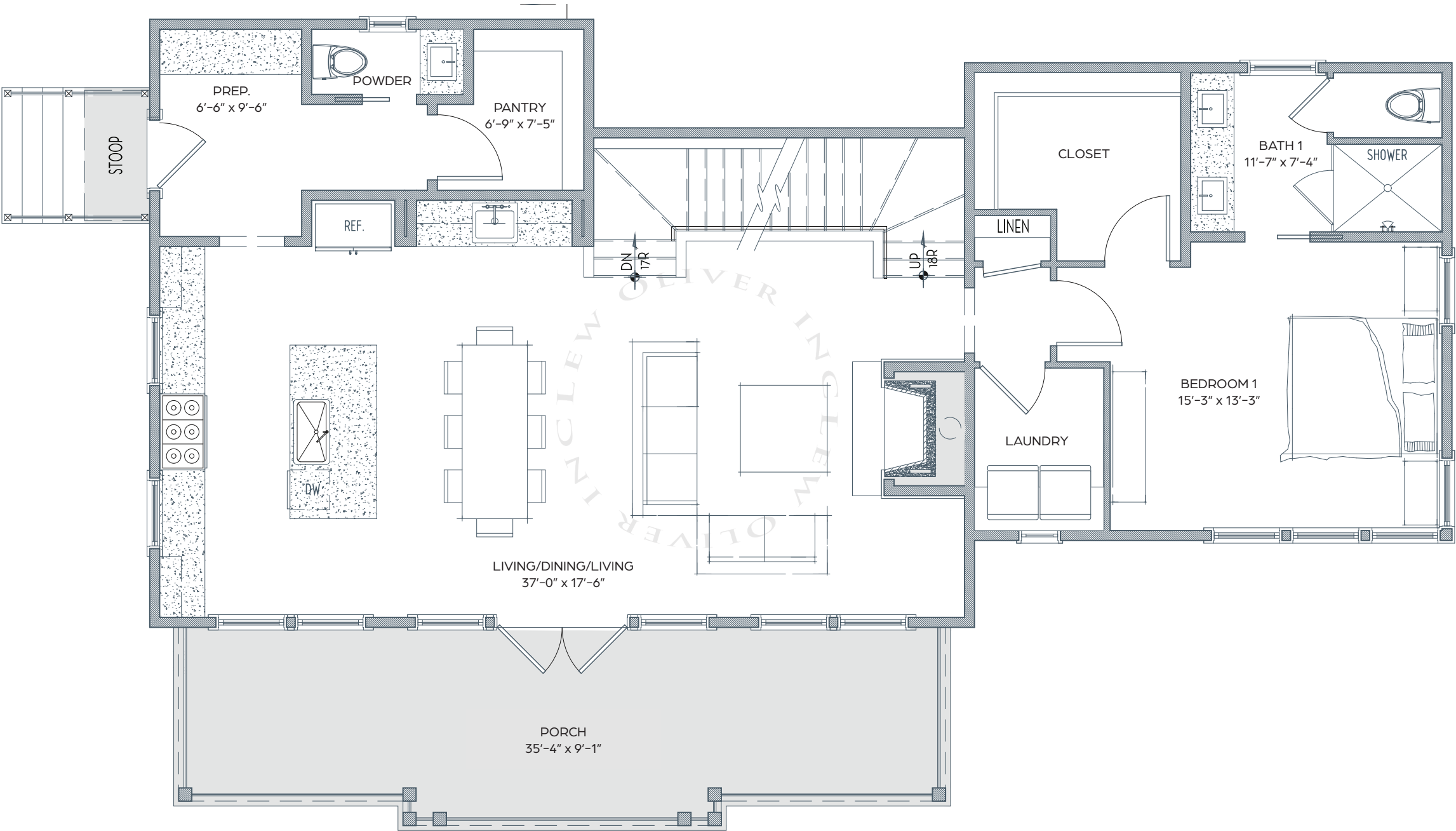
FIRST FLOOR
