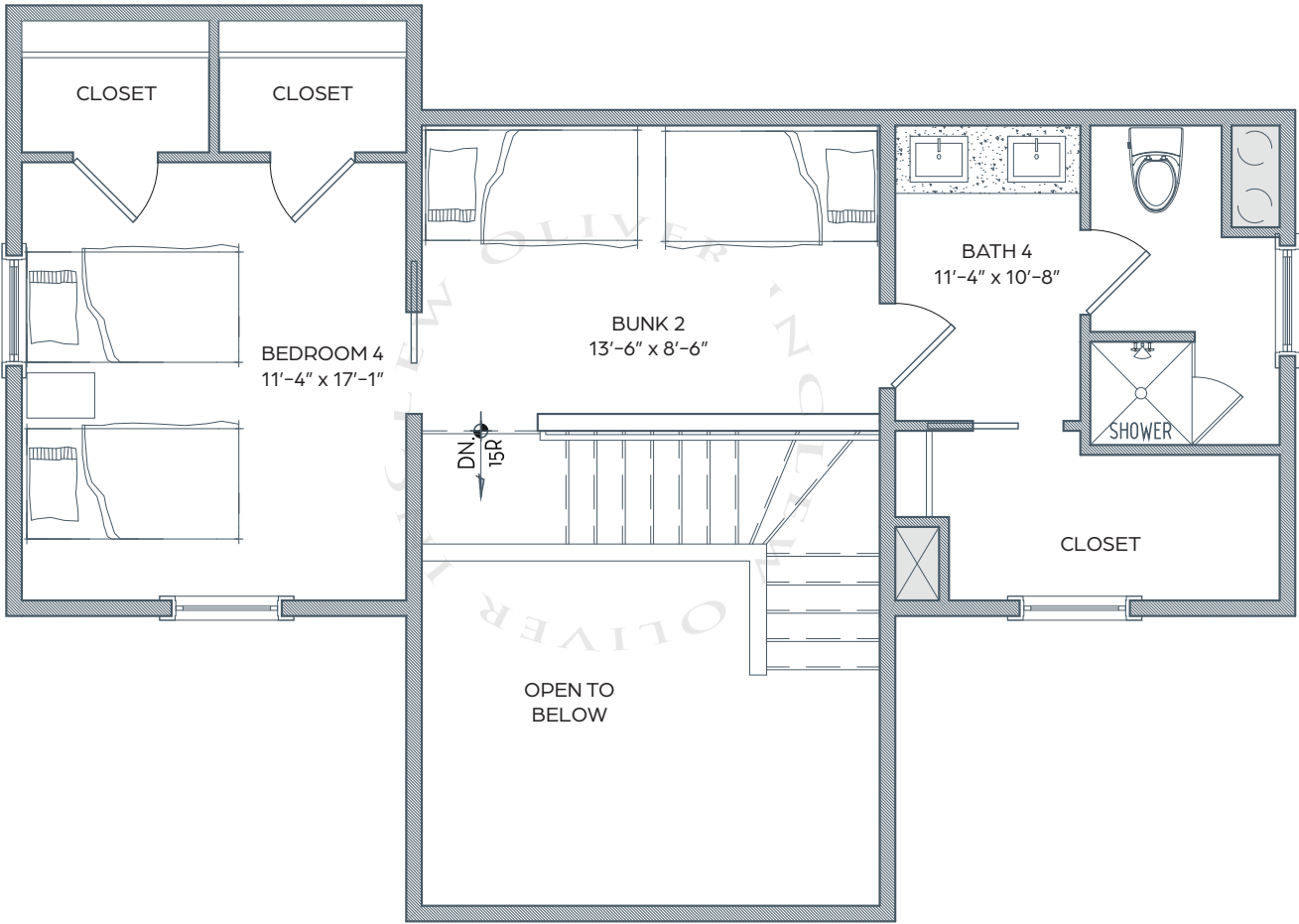
THIRD FLOOR
